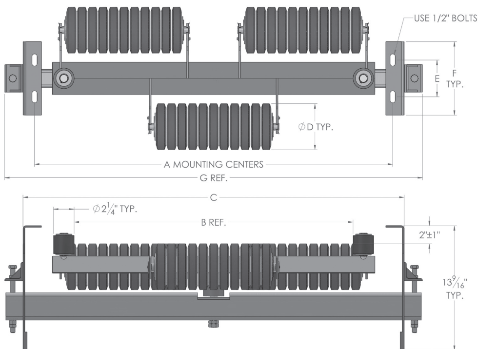
NEGOTIATOR™ SELF ALIGNING RETURN IDLER 5" RUBBER DISCS
